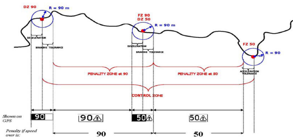
Diagram E - successive decreasing speed control zones from 90 to 50 kph
